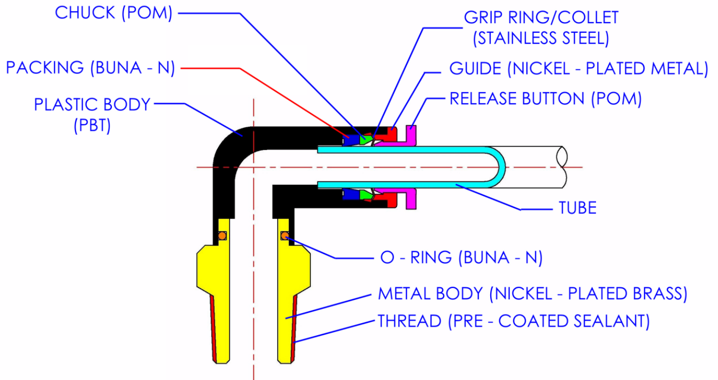
SCHMATIC OF TYPICAL COMPOSITE FITTING CONSTRUCTION
