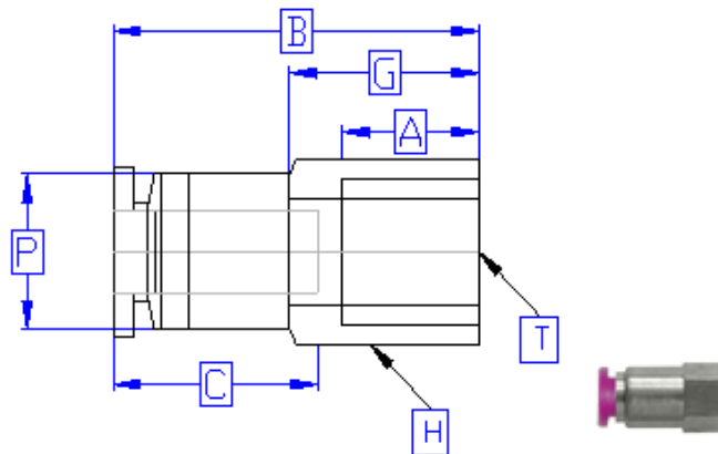
Female Connector
